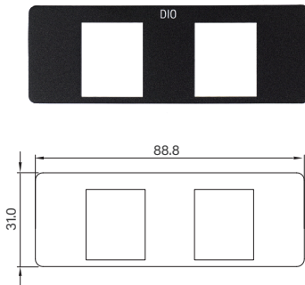
UB1018 Universal Bracket with DIO Cutout Dimension (WxD) : 88.8 x 31.0 mm
