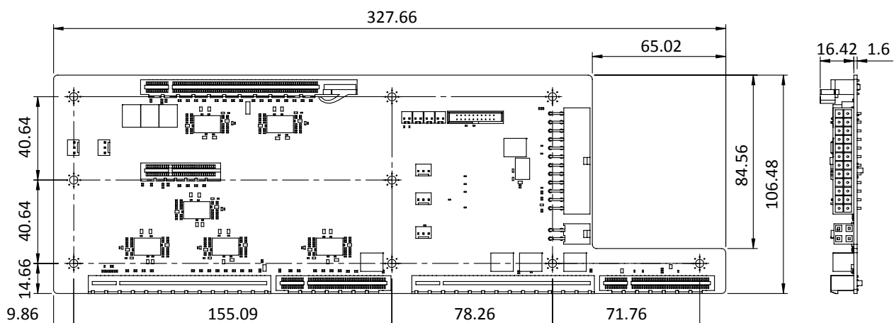
PE-3S1 Dimensions (Unit: mm)
