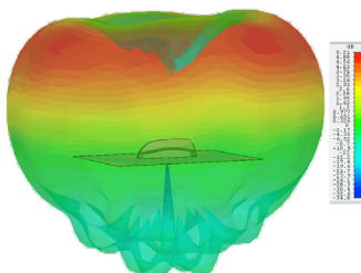
3D Gain Plot Side (1800MHz)
