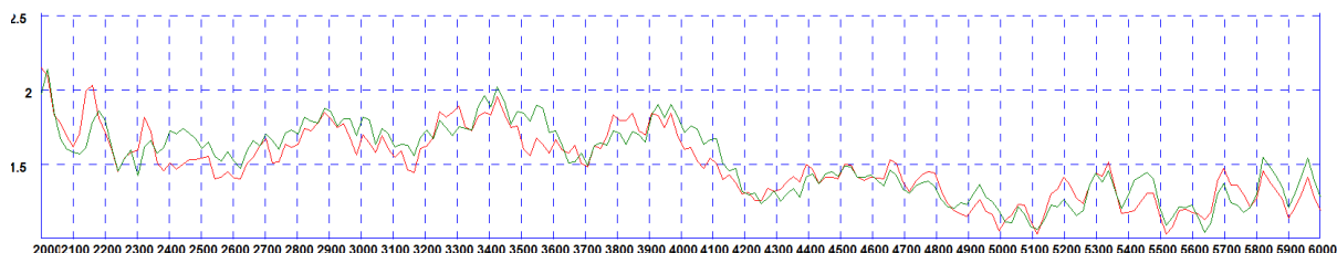
Typical VSWR - WiFi Elements 4&5*
