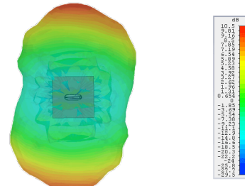
3D Gain Plot Top (3600MHz)
