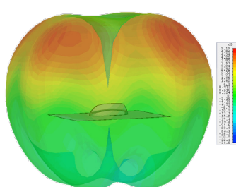
3D Gain Plot Side (900MHz)
