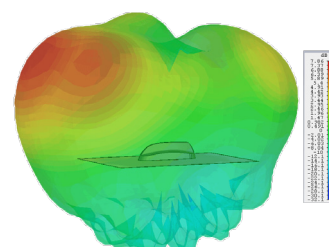
3D Gain Plot Side (2100MHz)
