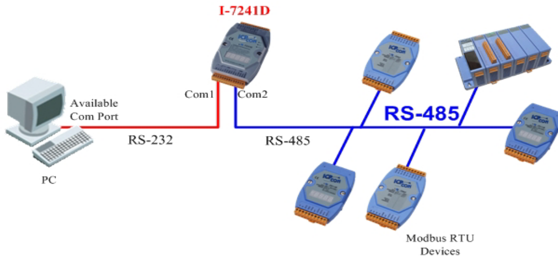
Fig 5-14. The configuration architecture of the I-7241D
