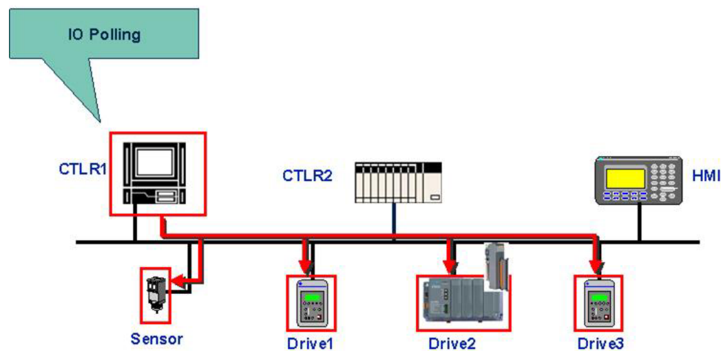
Figure 3.5 The architecture of IO bit strobe message
