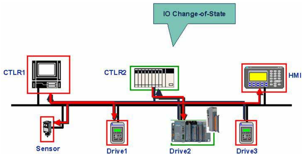
Figure 3.6 The architecture of IO COS message
