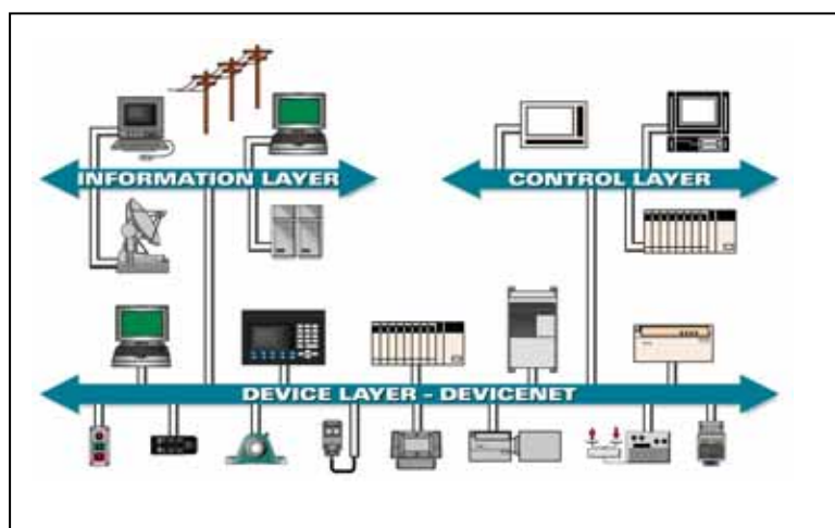
Figure 3.1 DeviceNet layer
