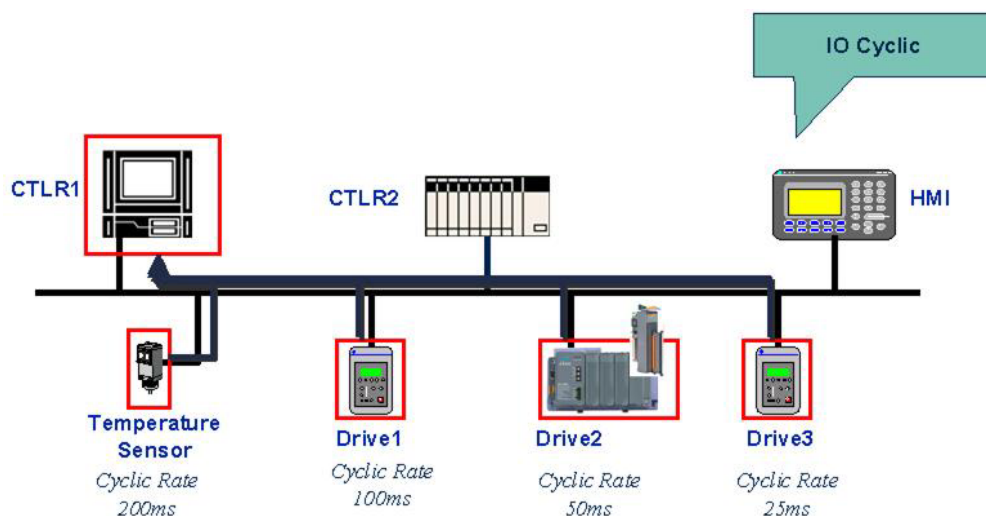
Figure 3.7 The architecture of IO Cyclic message
