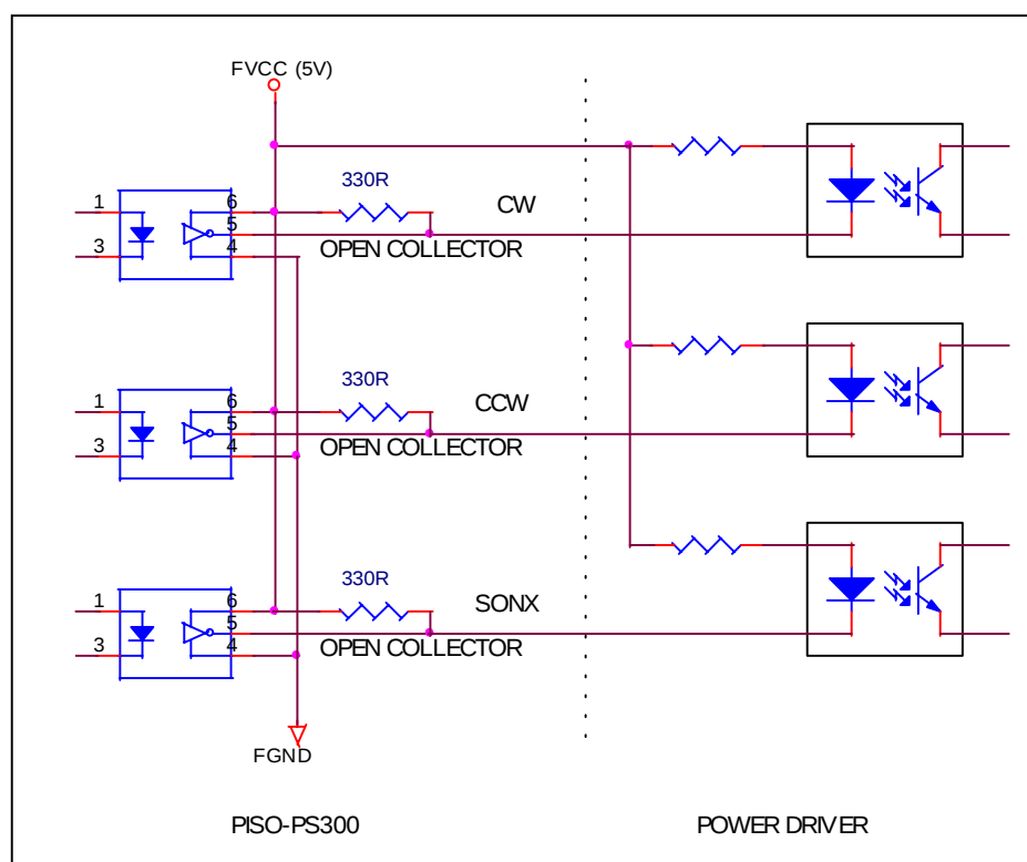
Sink type connection
