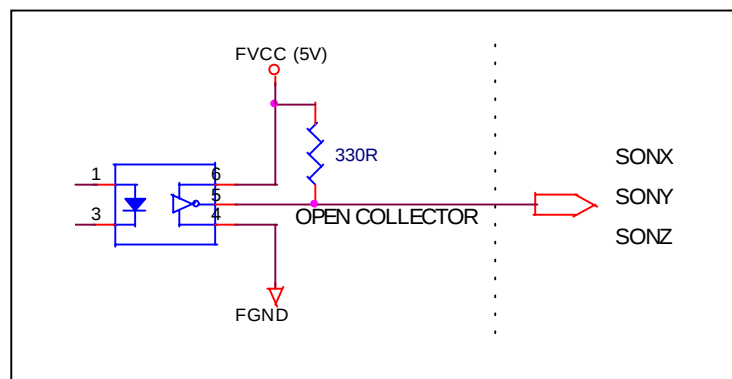
Figure(7) internal circuitry of Servo-ON signal
