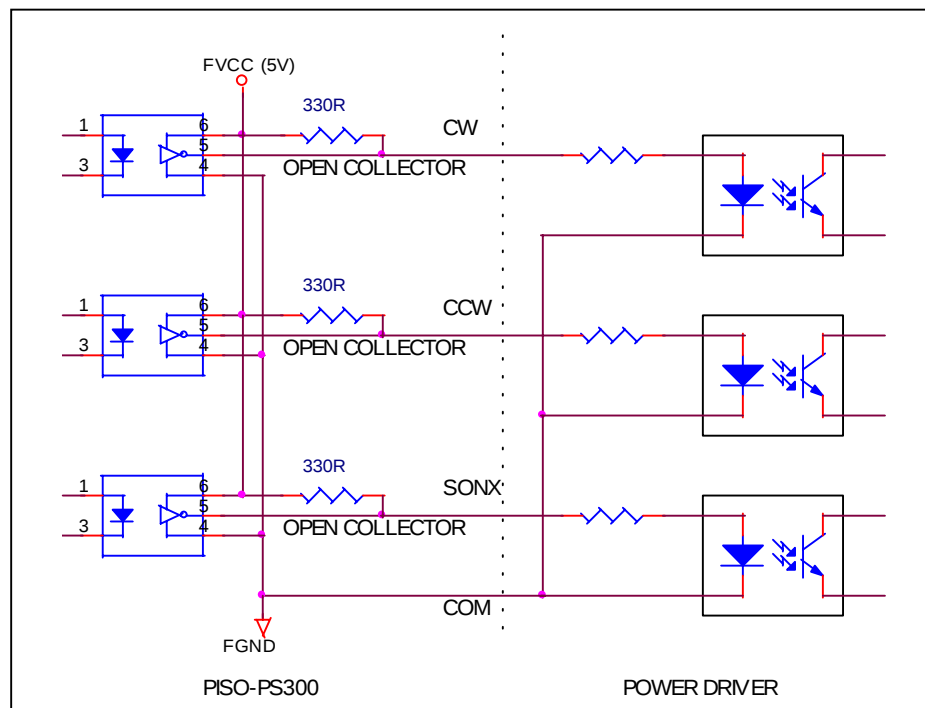
Source type connection
