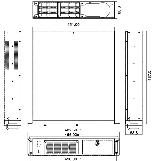
RACK-220GB B-Black
